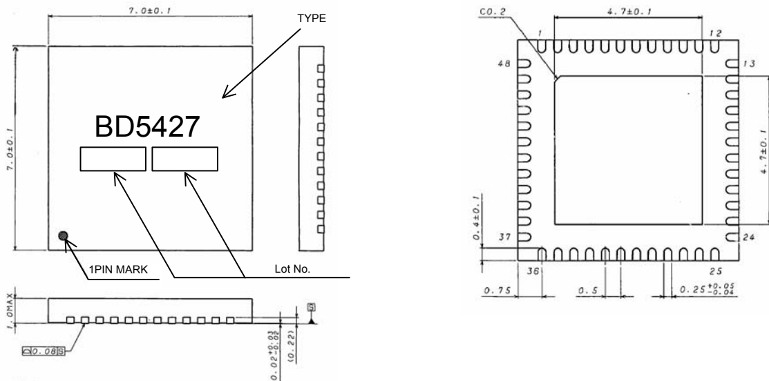
Fig. 23 Outer Dimensions and Incriptions of VQFN048V7070 Package
