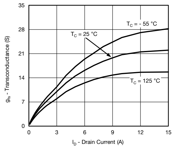
Transconductance
