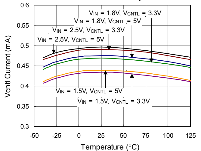
V cntl Current vs. Temperature
