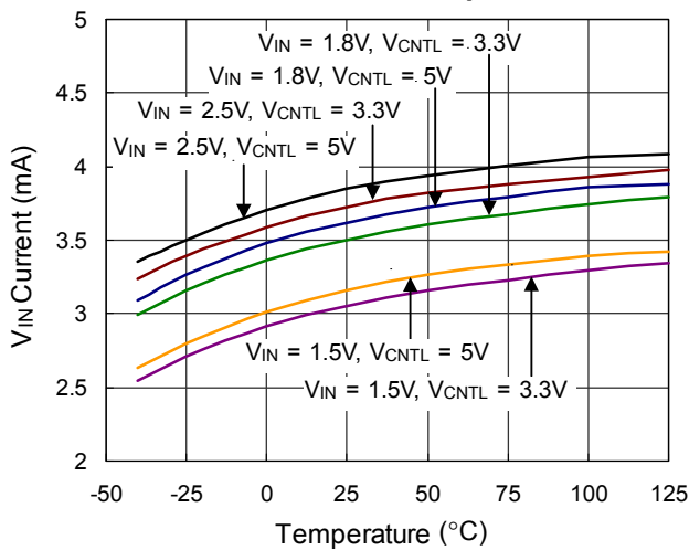
V IN Current vs. Temperature
