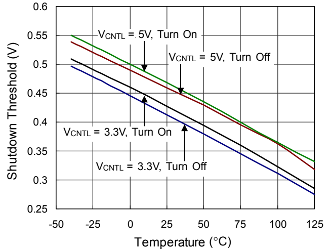
Shutdown Threshold vs. Temperature
