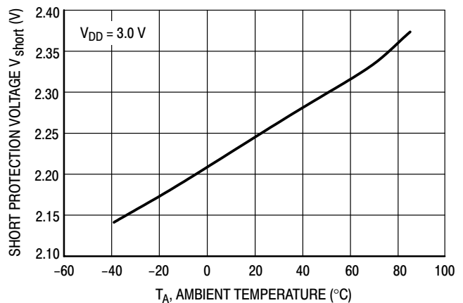
Figure 7. Short Protection Voltage vs Temperature MC33349N-3X
