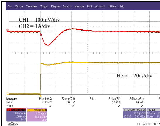
Vo=1.8V Typical output voltage transient response to load step from 25% to 75% of full load with output current slew rate of 10A/uS. (Cext = 1x100uF ceramic capacitor)
