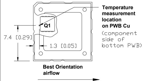
iCG12006A007V thermal measurement location – top view
