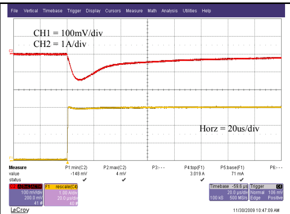
Vo=3.3V Typical output voltage transient response to load step from 0% to 50% of full load with output current slew rate of 10A/uS. (Cext = 1x100uF ceramic capacitor)
