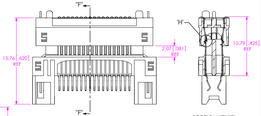
SECTION "F"-"F"
