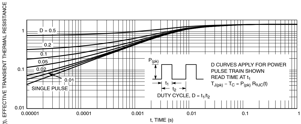
Figure 12. Thermal Response
