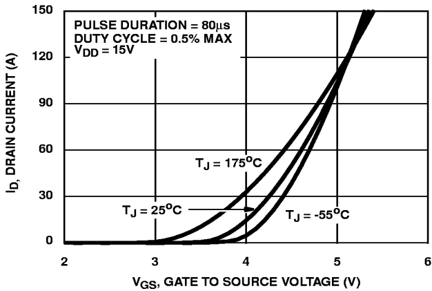
FIGURE 7. TRANSFER CHARACTERISTICS
