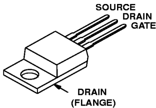
HUF75545P3
