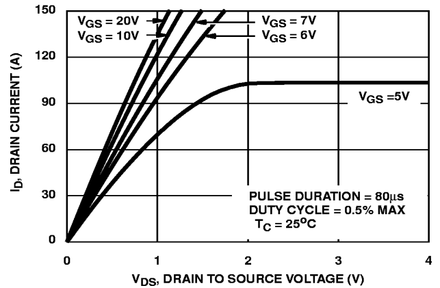
FIGURE 8. SATURATION CHARACTERISTICS
