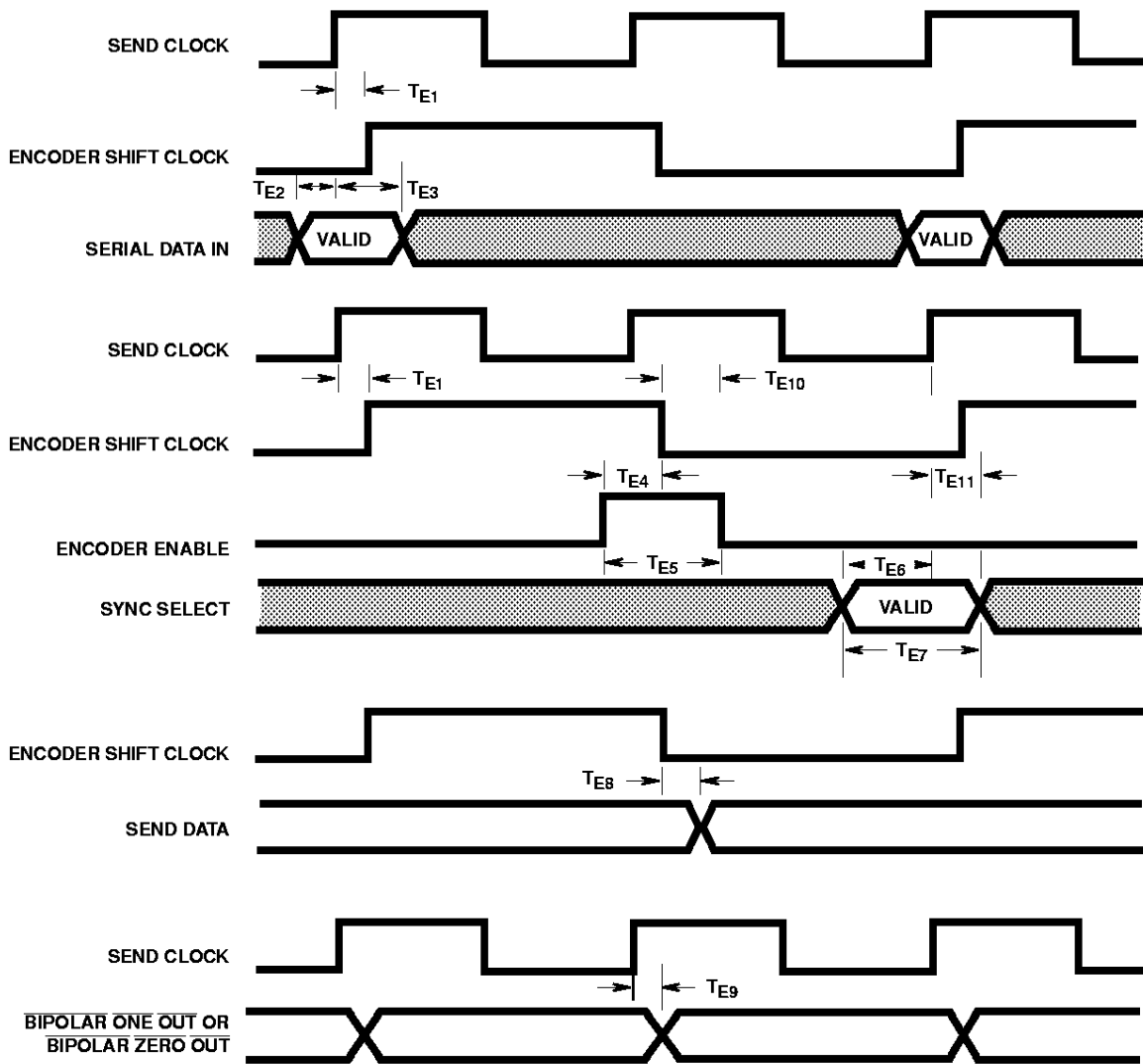
FIGURE 10. ENCODER TIMING
