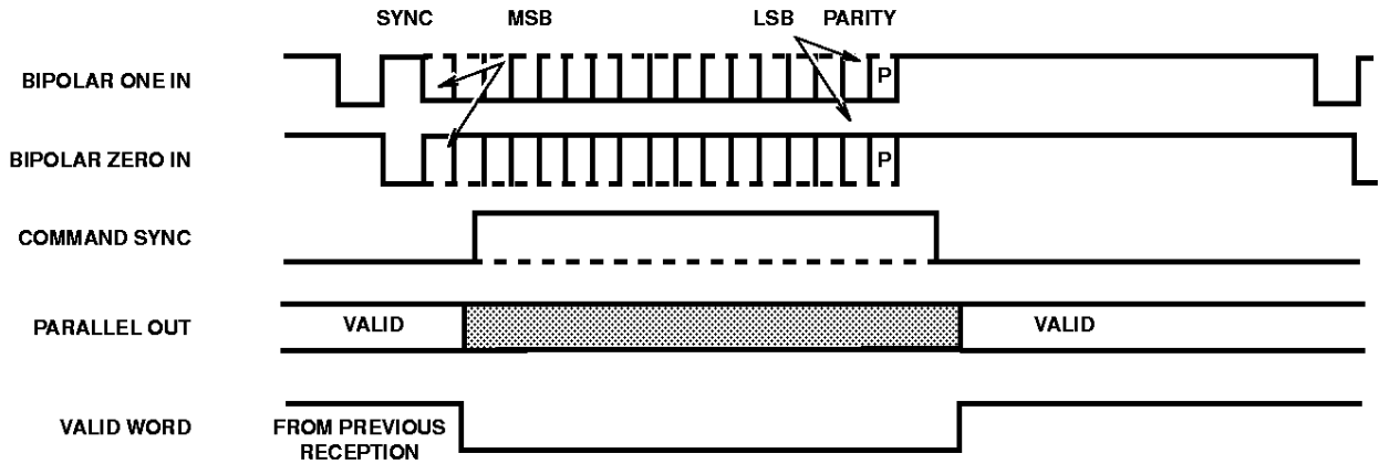
FIGURE 5. DECODER TIMING
