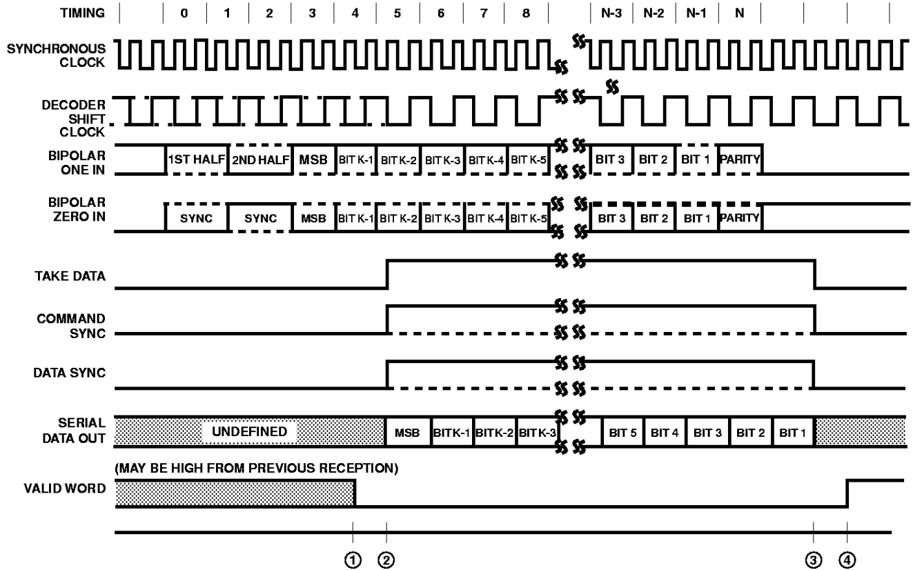
FIGURE 2. DECODER
