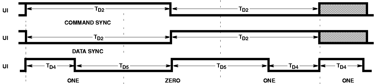
FIGURE 11. DECODER TIMING
