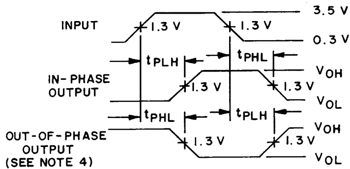
VOLTAGE WAVEFORMS PROPAGATION DELAY TIMES
