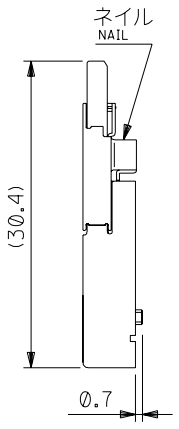
詳細 D DETAIL D (SCALE 5:1)
