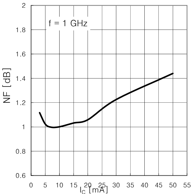
NF vs. I_C V_{CE} = 3 V, I_C = \text{parameter}, Z_S = Z_{Sopt}
