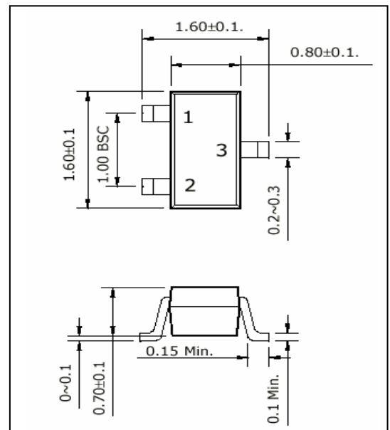
SOT 523 Unit in mm
