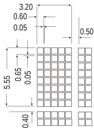
DISPLAY PATTERN DIMENSIONS
