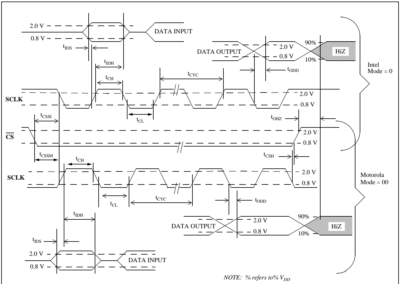
Figure 14 - Microport Timing
