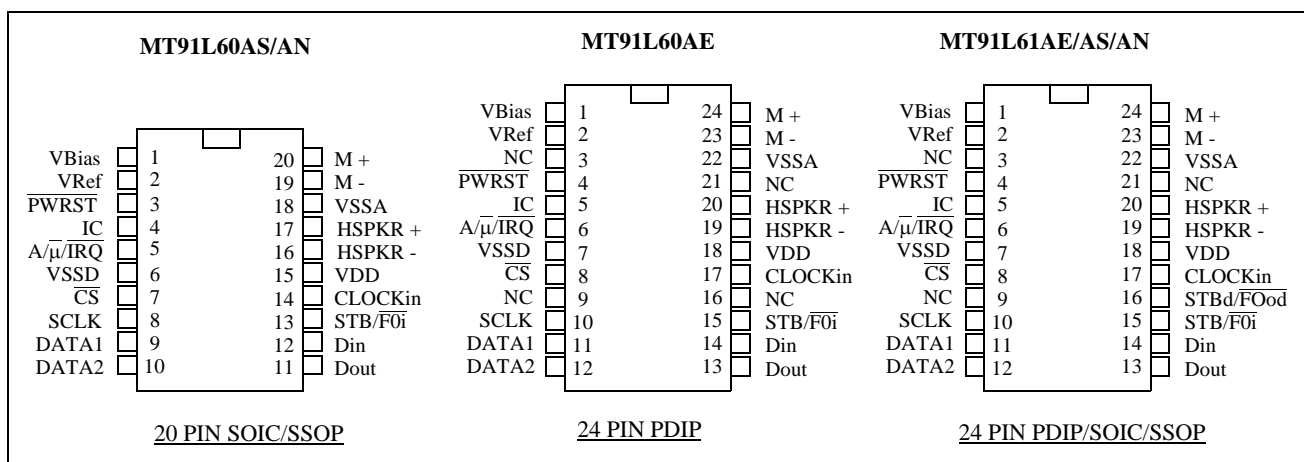
Figure 2 - Pin Connections
