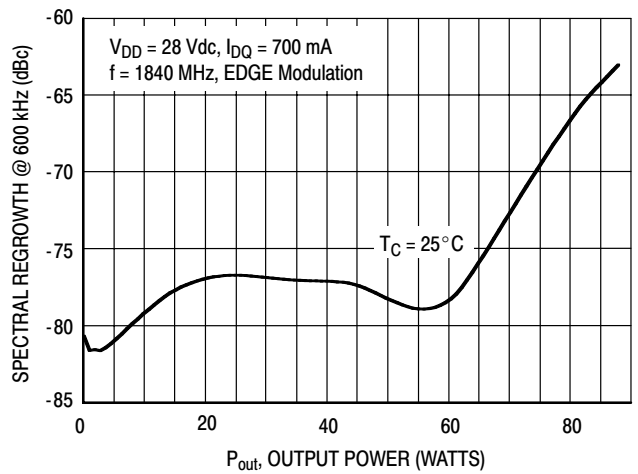
Figure 24. Spectral Regrowth at 600 kHz versus Output Power
