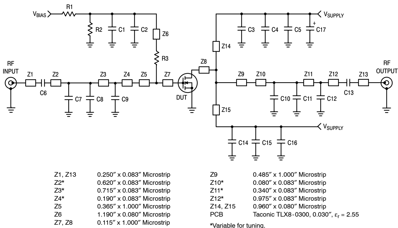
Figure 16. MRF6S18100NR1(NBR1) Test Circuit Schematic — 1805-1880 MHz
