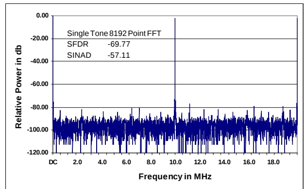
Figure 5 - FFT Spectrum @ F_{clock} = 40.0\text{MHz} , F_{in} = 10.0\text{MHz} , DIFFERENTIAL INPUT MODE
