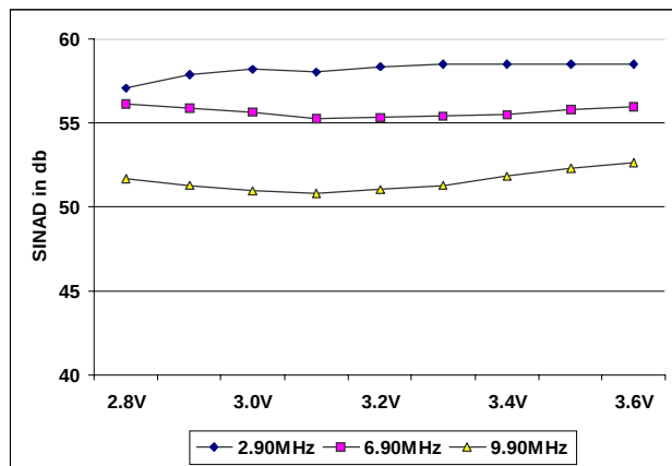
Figure 6 - SINAD vs. F_{in} and V_{dd} @ F_c = 40.0\text{MHz} , SINGLE-ENDED INPUT MODE
