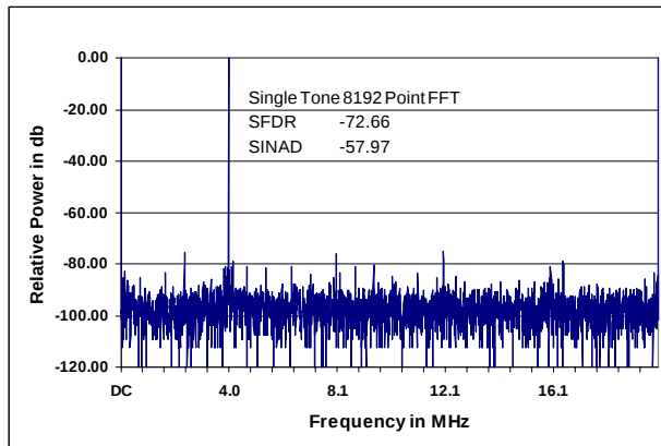
Figure 4 - FFT Spectrum @ F_{clock} = 40.0\text{MHz} , F_{in} = 4.0\text{MHz} , DIFFERENTIAL INPUT MODE
