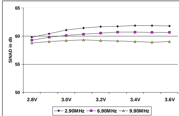
Figure 2 - SINAD vs. F_{in} and V_{dd} @ F_c = 40.0\text{MHz} , DIFFERENTIAL INPUT MODE
