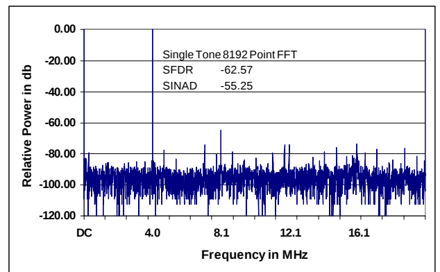
Figure 7 - FFT Spectrum @ F_{clock} = 40.0\text{MHz} , F_{in} = 4.0\text{MHz} , Single-ended INPUT MODE
