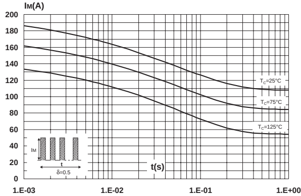
Fig. 3-1: Non repetitive surge peak forward current versus overload duration (maximum values) (TO-220AB, D 2 PAK, I 2 PAK).
