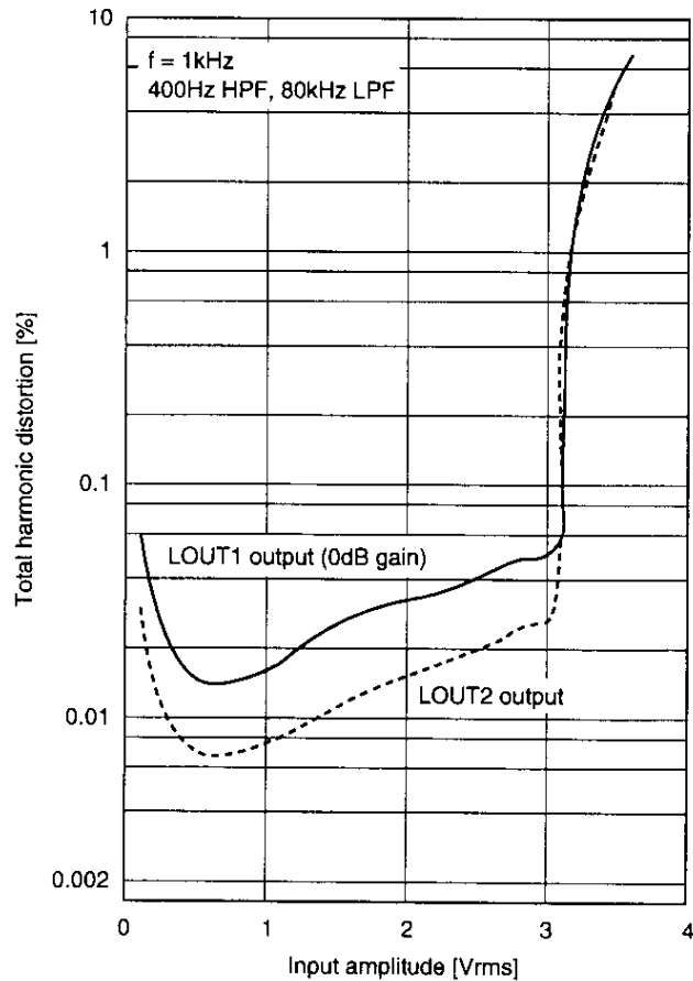
Audio system distortion vs. Input amplitude
