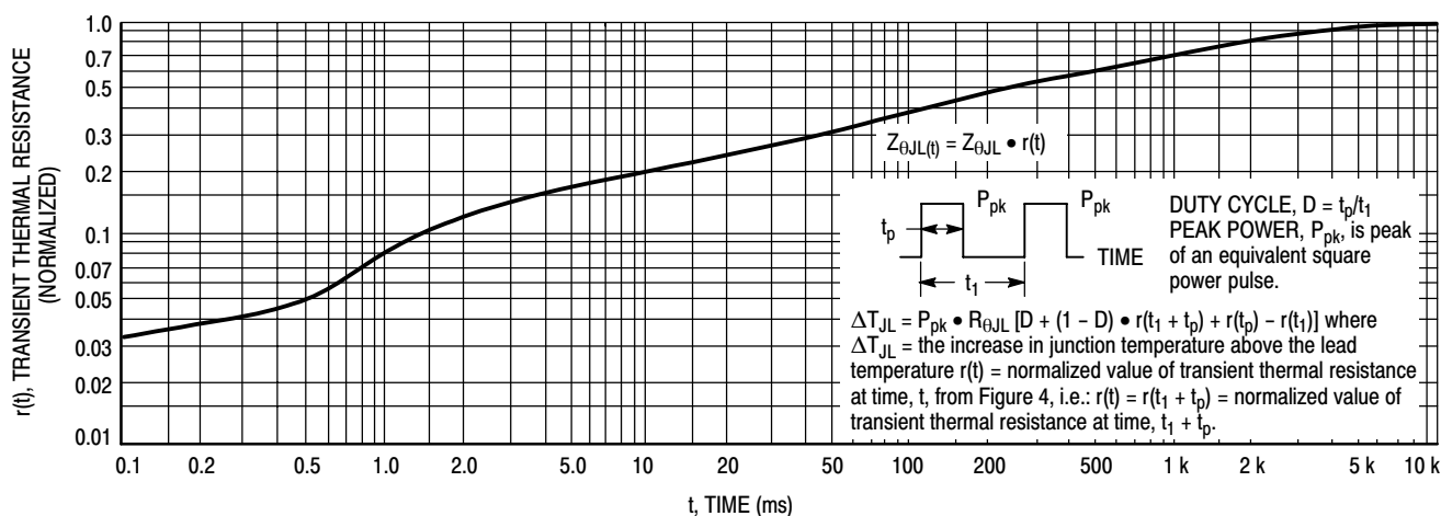
Figure 4. Thermal Response
