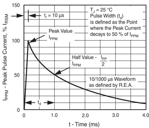
Fig. 3 - Pulse Waveform
