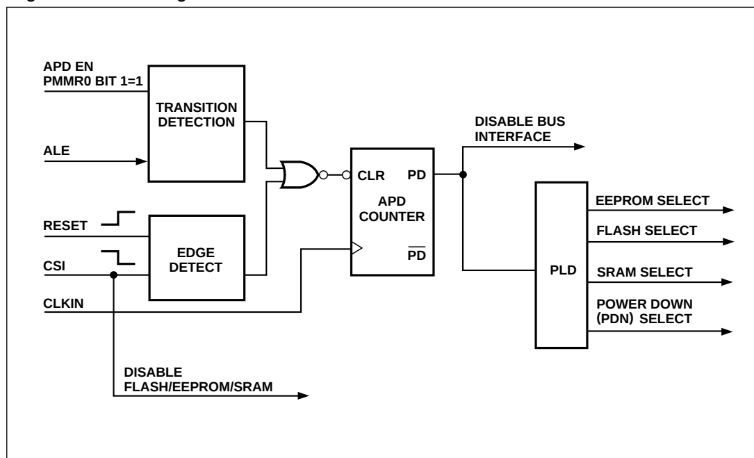
Figure 25. APD Logic Block
