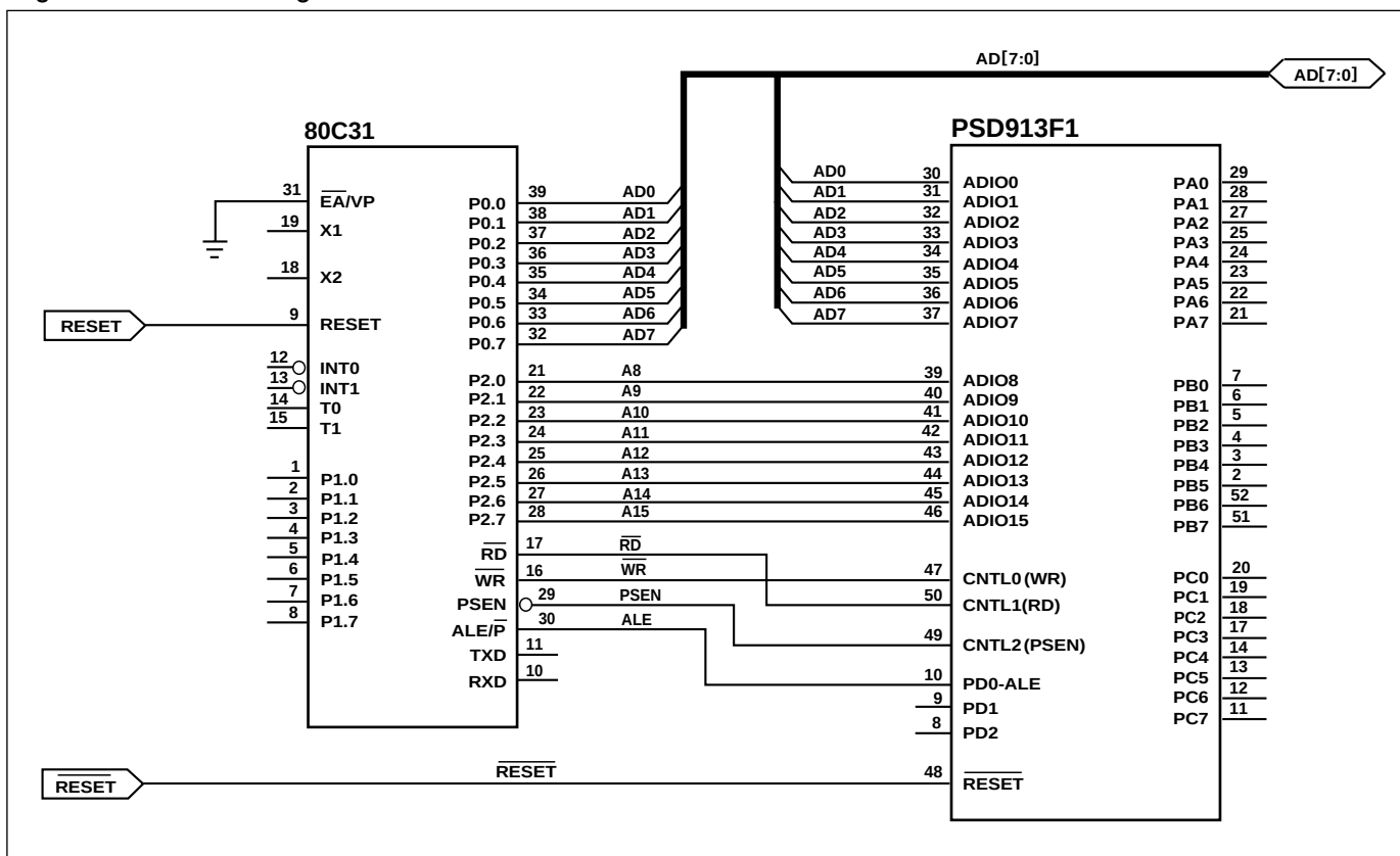
Figure 16. Interfacing the PSD913F1 with an 80C31
