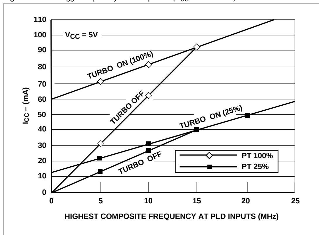
Figure 28. PLD I_{CC} /FrequencyConsumption ( V_{CC} = 5\text{ V} \pm 10\% )
