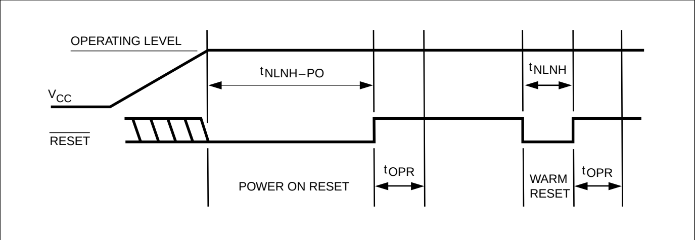
Figure 33. Reset Timing
