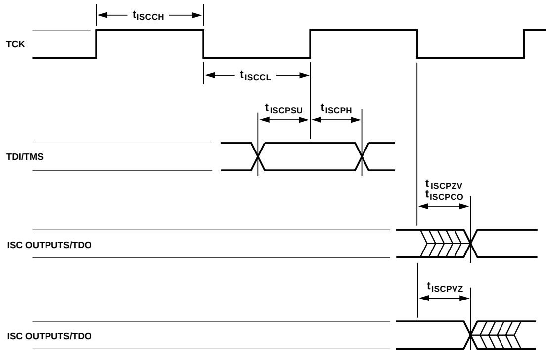
Figure 32. ISC Timing
