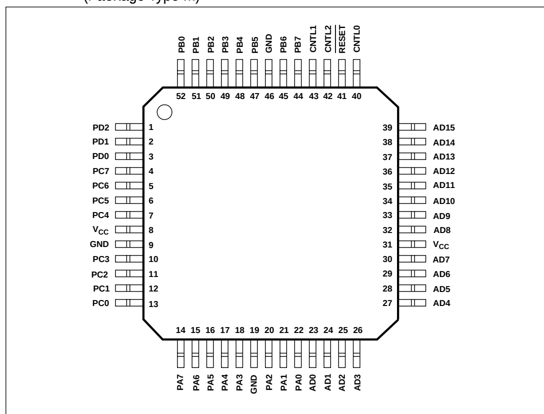
Figure 38. Drawing M3 – 52-Pin Plastic Quad Flatpack (PQFP) (Package Type M)
