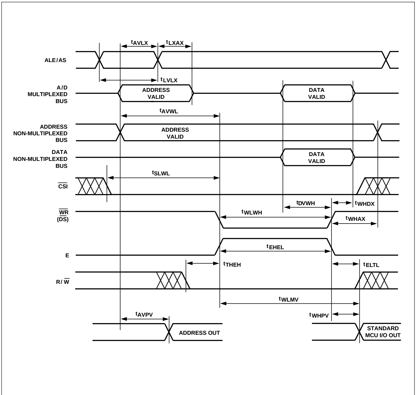
Figure 30. Write Timing
