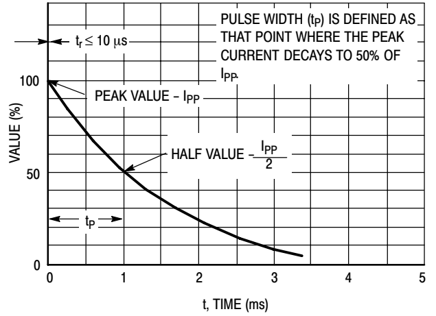
Figure 2. Pulse Waveform
