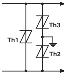
Figure 32. MULTI-POINT PROTECTION
