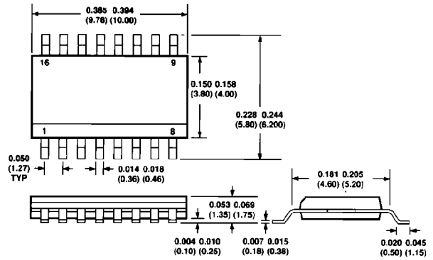
16-Pin SOIC
