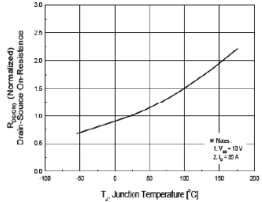
Fig.8 On-Resistance Variation vs. Junction temperature
