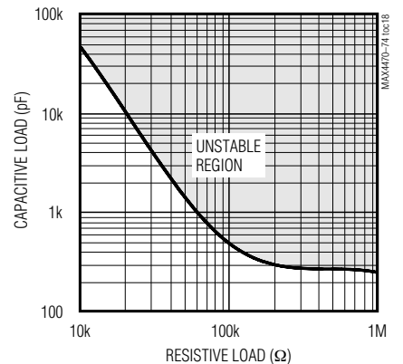
MAX4470/MAX4471/MAX4472 STABILITY vs. CAPACITIVE AND RESISTIVE LOADS
