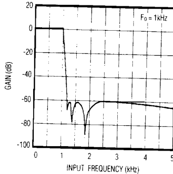
MAX294 PASSBAND FREQUENCY RESPONSE
