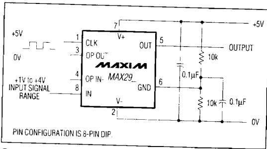
Figure 3. +5V Single-Supply Operation
