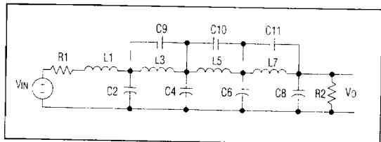
Figure 2. 8th-Order Ladder Filter Network
