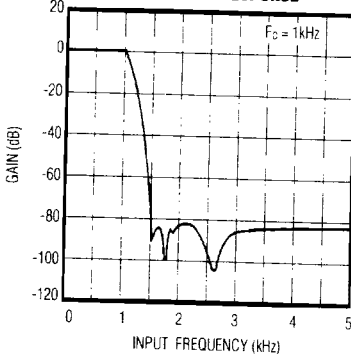
MAX293 PASSBAND FREQUENCY RESPONSE
