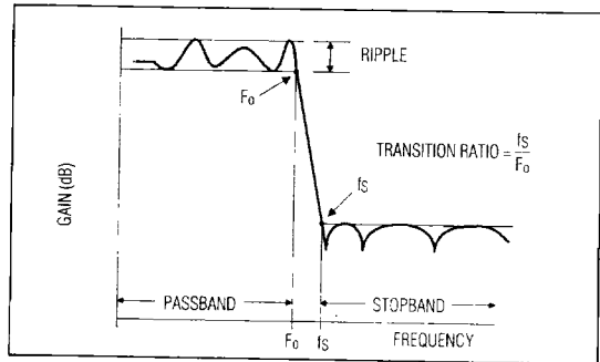
Figure 1. Elliptic Filter Response
