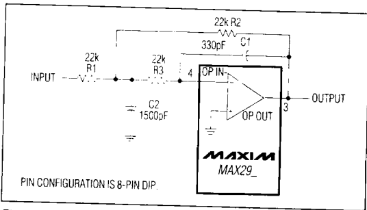
Figure 4. Uncommitted Op Amp Configured as a 2nd-Order Butterworth Lowpass Filter ( F_o = 10\text{kHz} )
