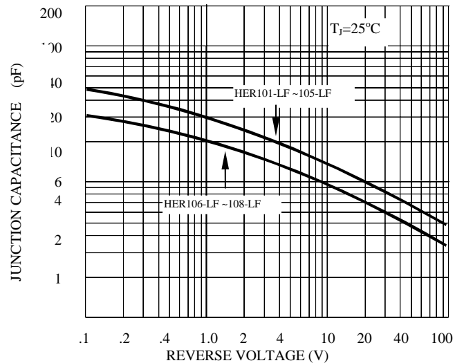
FIG. 6-TYPICAL JUNCTION CAPACITANCE
