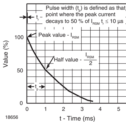
Fig. 2 - Pulse Waveform
