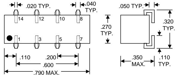
MDU3C-xxB2 (Commercial J-Lead)
