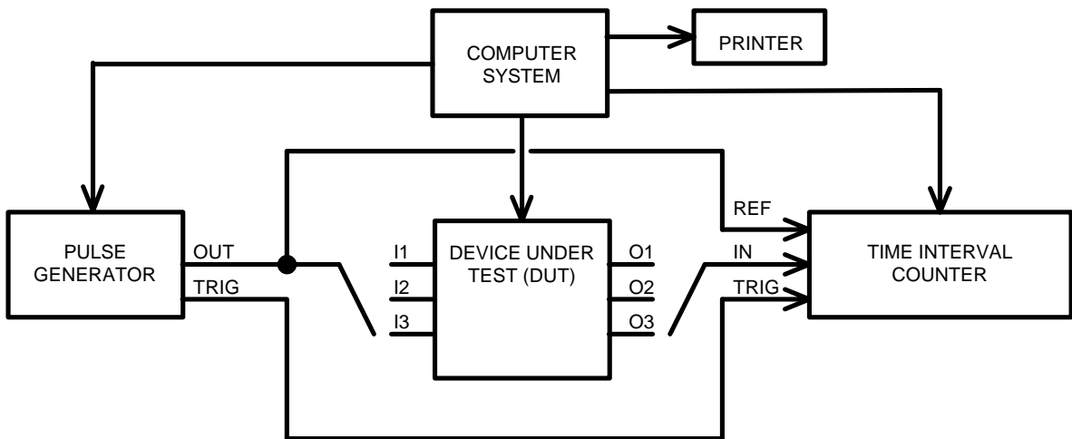
Test Setup
