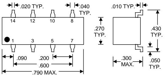
MDU3C-xxA2 (Commercial Gull-Wing)
