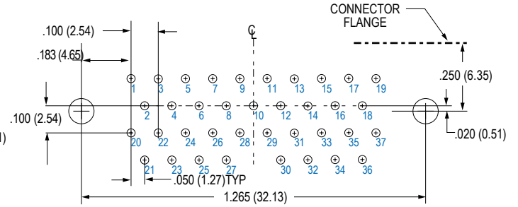
37 PIN M83513/10-F
