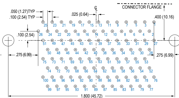
100 SOCKET M83513/15-H
