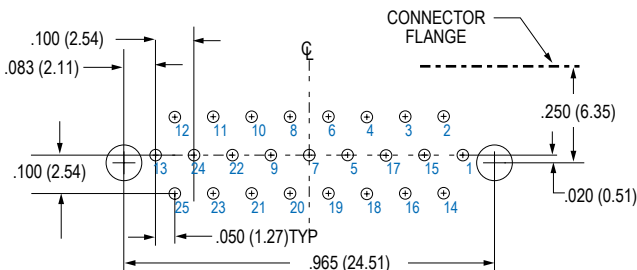
25 SOCKET M83513/13-D
