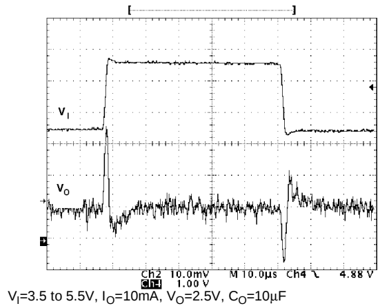
Figure 15 : Line Transient
