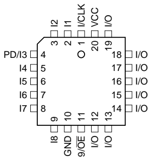
PLCC
