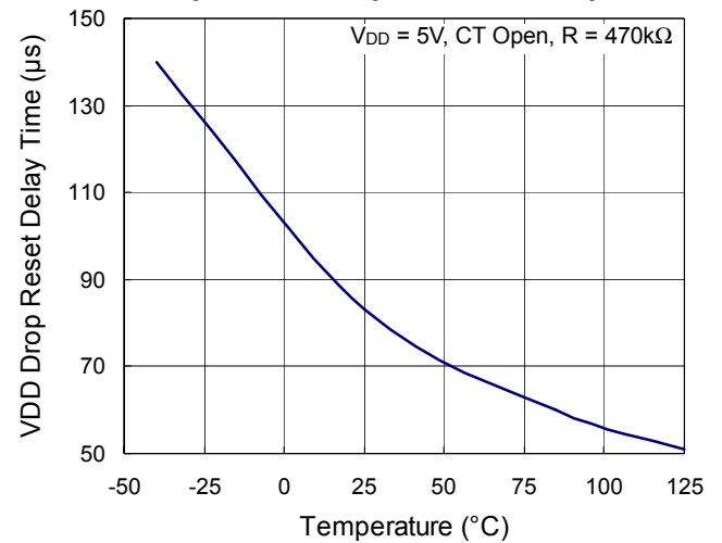
VDD Drop Reset Delay Time vs. Temperature
