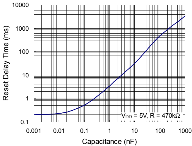
Reset Delay Time vs Capacitance
