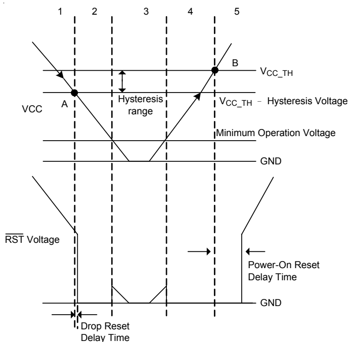
Figure 3. Operation Diagram
