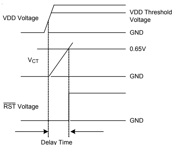
Figure 1. Delay Time
