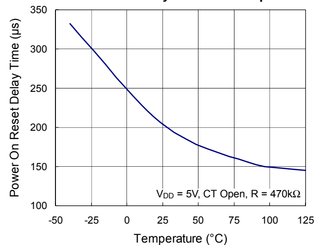
Power On Reset Delay Time vs. Temperature
