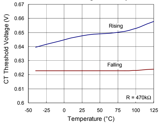
CT Threshold Voltage vs. Temperature
