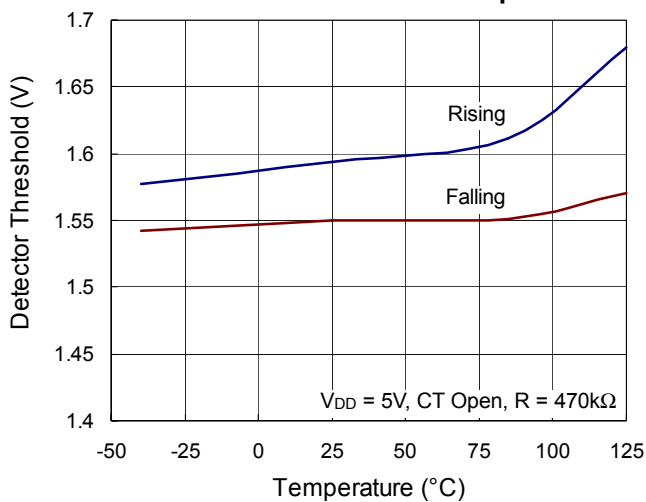
Detector Threshold vs. Temperature
