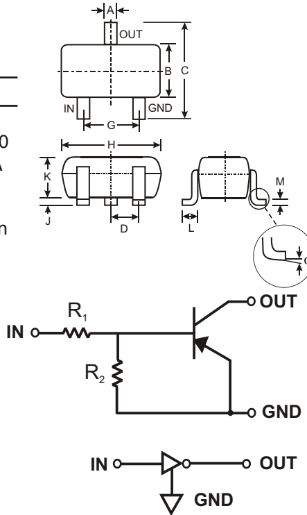
SCHMATIC DIAGRAM
