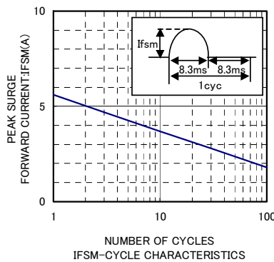
IFSM-CYCLE CHARACTERISTICS
