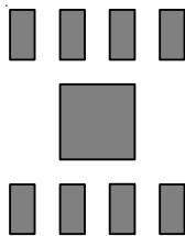
(a) Copper Area = (2.3 x 2.3) mm², \theta_{JA} = 75^{\circ}\text{C/W}
