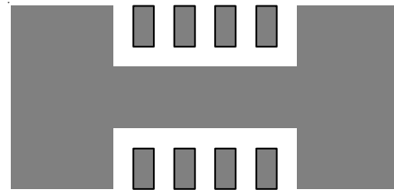
(e) Copper Area = 70mm², \theta_{JA} = 49^{\circ}\text{C/W}
