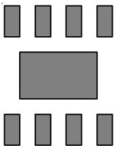
(b) Copper Area = 10mm², \theta_{JA} = 64^{\circ}\text{C/W}
