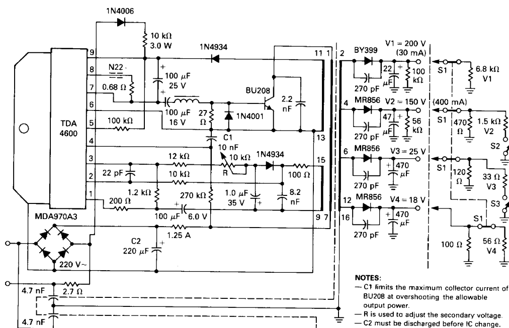
FIGURE 7 — TYPICAL APPLICATION
