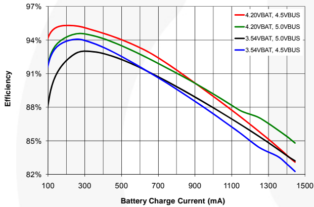
Figure 9. Charger Efficiency, No I_{INLIM} , I_{CHARGE}=1,450mA
