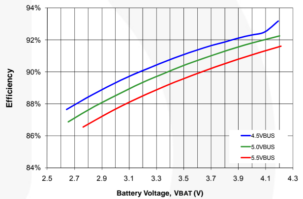
Figure 10. Charger Efficiency vs. V_{BUS} , I_{INLIM}=500mA
