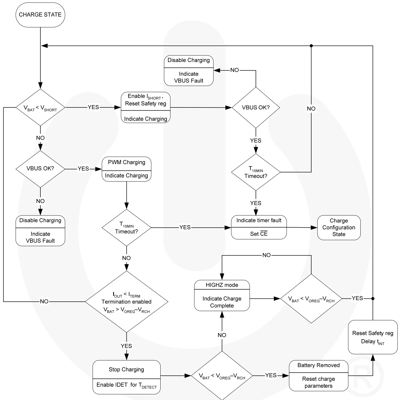
Figure 38. Charge Mode
