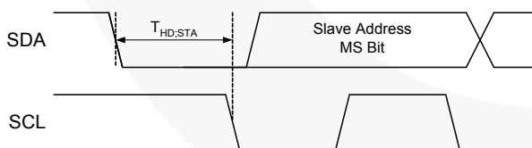
Figure 46. Start Bit
