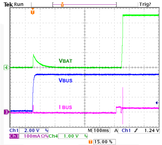
Figure 18. No Battery at V_{BUS} Power-up; FAN54012, FAN54015
