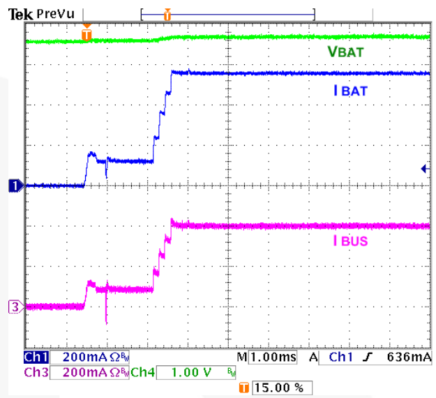
Figure 14. Charger Startup with HZ_MODE Bit Reset, I_{NLIM}=500mA , I_{OCHARGE}=1,050mA , OREG=4.2V , V_{BAT}=3.6V
