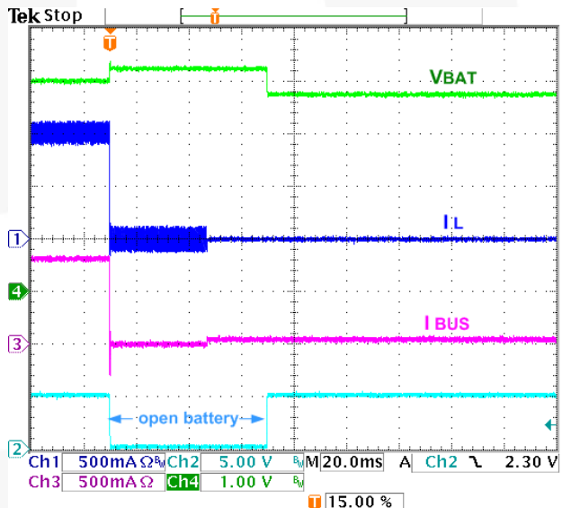
Figure 16. Battery Removal / Insertion During Charging, V_{BAT}=3.9V , I_{OCHARGE}=1,050mA , No I_{NLIM} , TE=1
