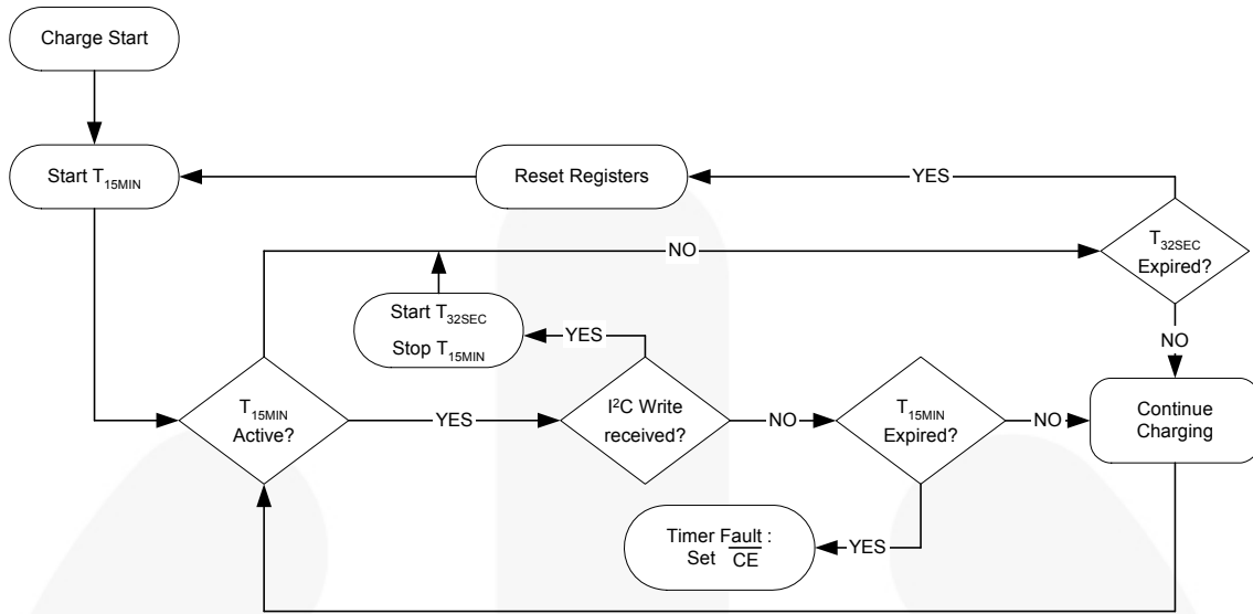
Figure 41. Timer Flow Chart for FAN54010, FAN54012, FAN54013, FAN54015
