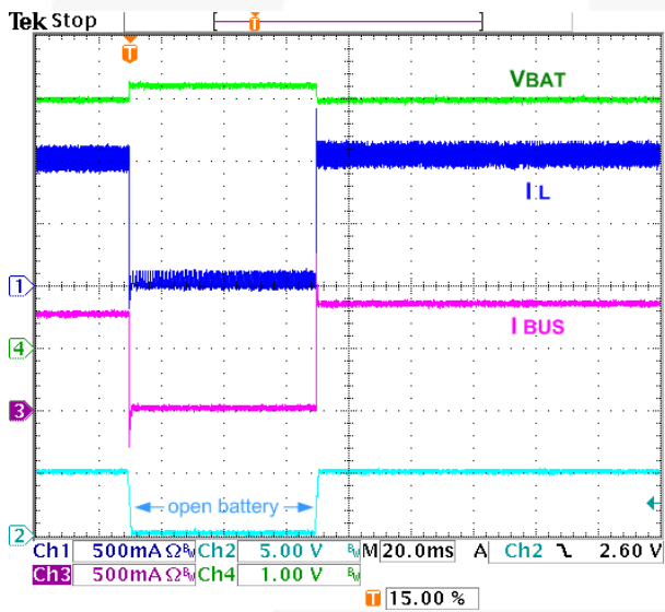
Figure 15. Battery Removal / Insertion During Charging, V_{BAT}=3.9V , I_{OCHARGE}=1,050mA , No I_{NLIM} , TE=0
