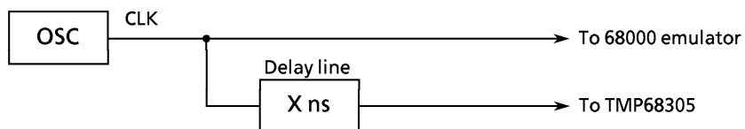
Figure 11.5 Clock Adjustments for Emulation
