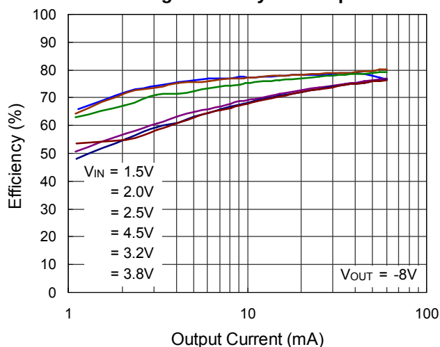
CH5 Inverting Efficiency vs. Output Current
