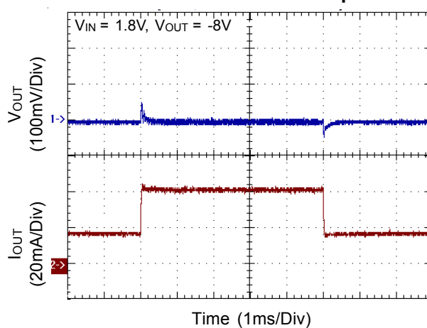
CH5 Load Transient Response
