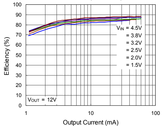
CH4 Boost Efficiency vs. Output Current
