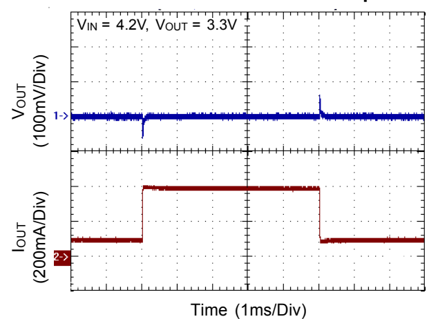
CH1 Buck Load Transient Response
