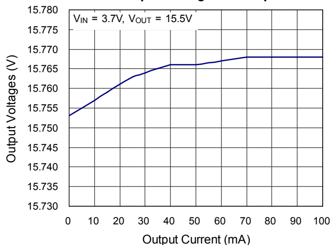
CH4 Boost Output Voltage vs. Output Current
