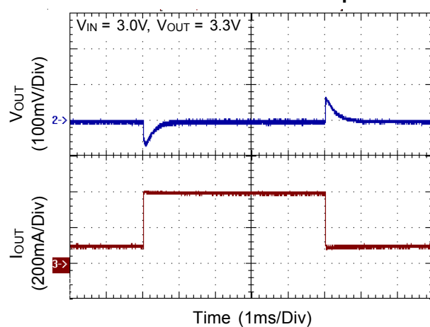
CH3 Load Transient Response
