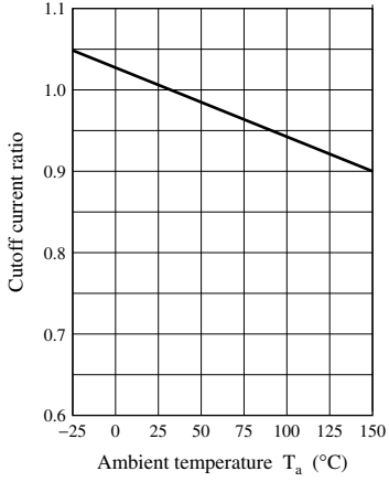
Cutoff current ratio — T_a
