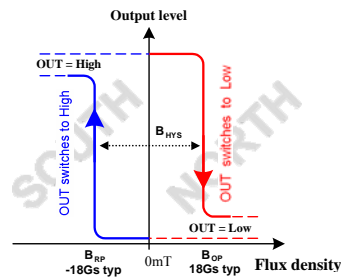
SO package - Latch characteristic
