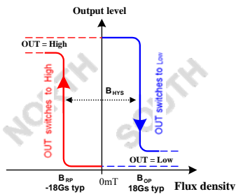
UA package - Latch characteristic
