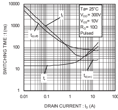
Fig. 14 Switching Characteristics
