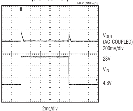
LINE-TRANSIENT RESPONSE (3.3V OUTPUT)
