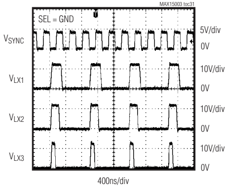
IN-PHASE OPERATION
