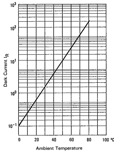
FIG. 4 DARK CURRENT VS. AMBIENT TEMPERATURE V_A = 10 , E_e = 0
