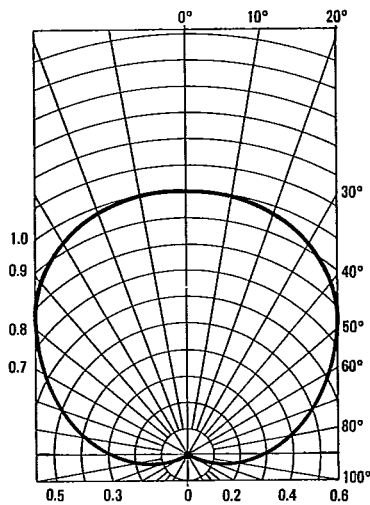
FIG. 7 SENSITIVITY DIAGRAM
