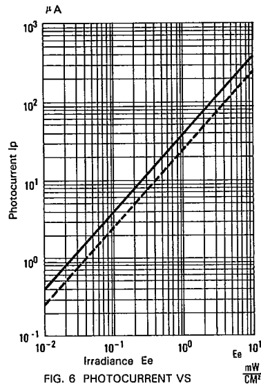
FIG. 6 PHOTOCURRENT VS IRRADIANCE = 950 NM
