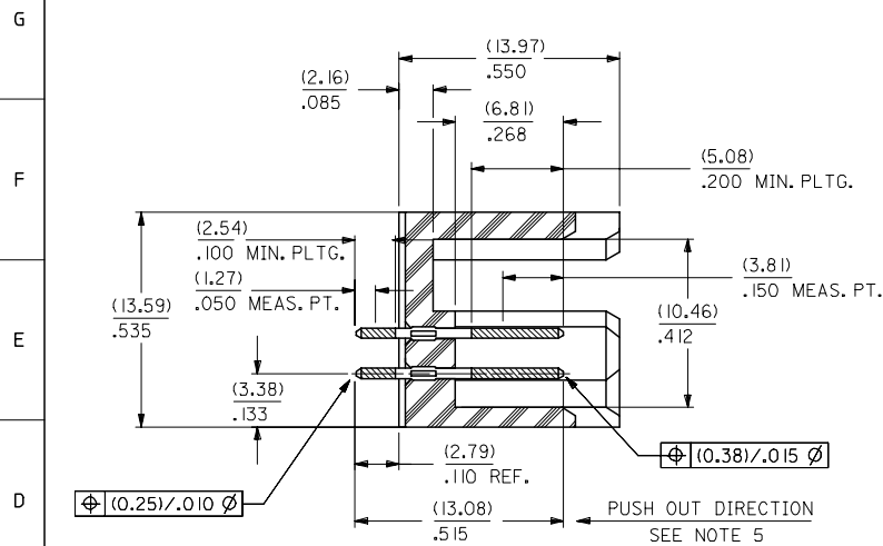
SECTION W-W
