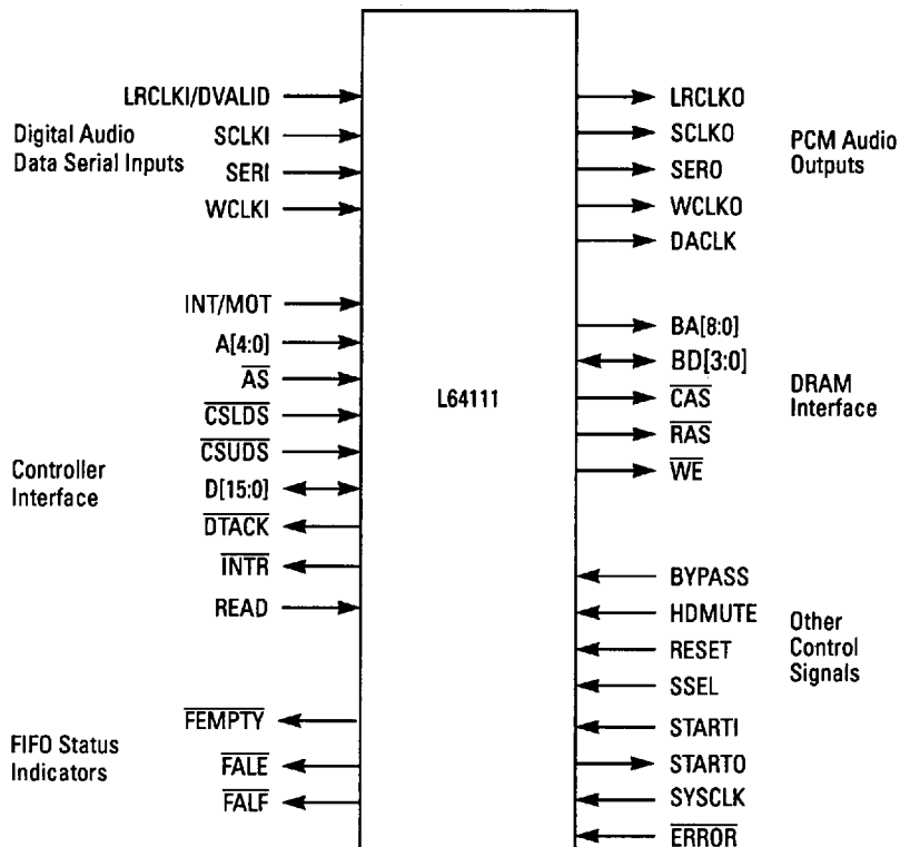
Figure 3.1 L64111 Logic Symbol
