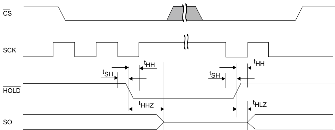
Figure 35. \overline{HOLD} Timing
